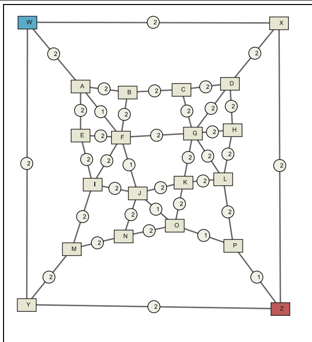
Initial graph
