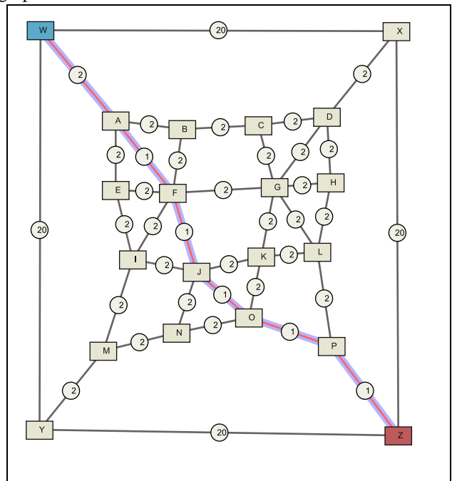
Shortest path after a modification of weight
