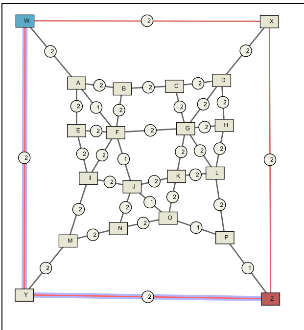
Shortest path
